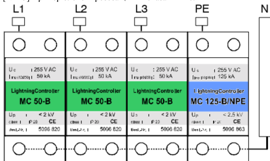
Circuit for TN-S, TT and IT systems
